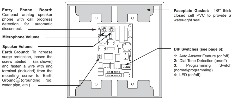
Rear (PCB) View of E-60
