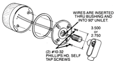
REAR MOUNTING TO ADAPTER PLATE
